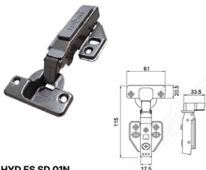
HYD ES SD 01N FULL OVERLAY TN
