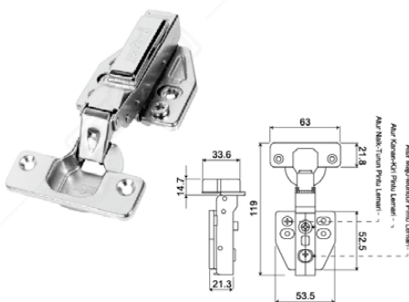
HYD ES SD D8383 3D ADJ HALF OVERLAY SN
