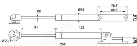
SPRING SUPPORT SPS 8152 - 100N SILVER (WITH SOFT CLOSER)
